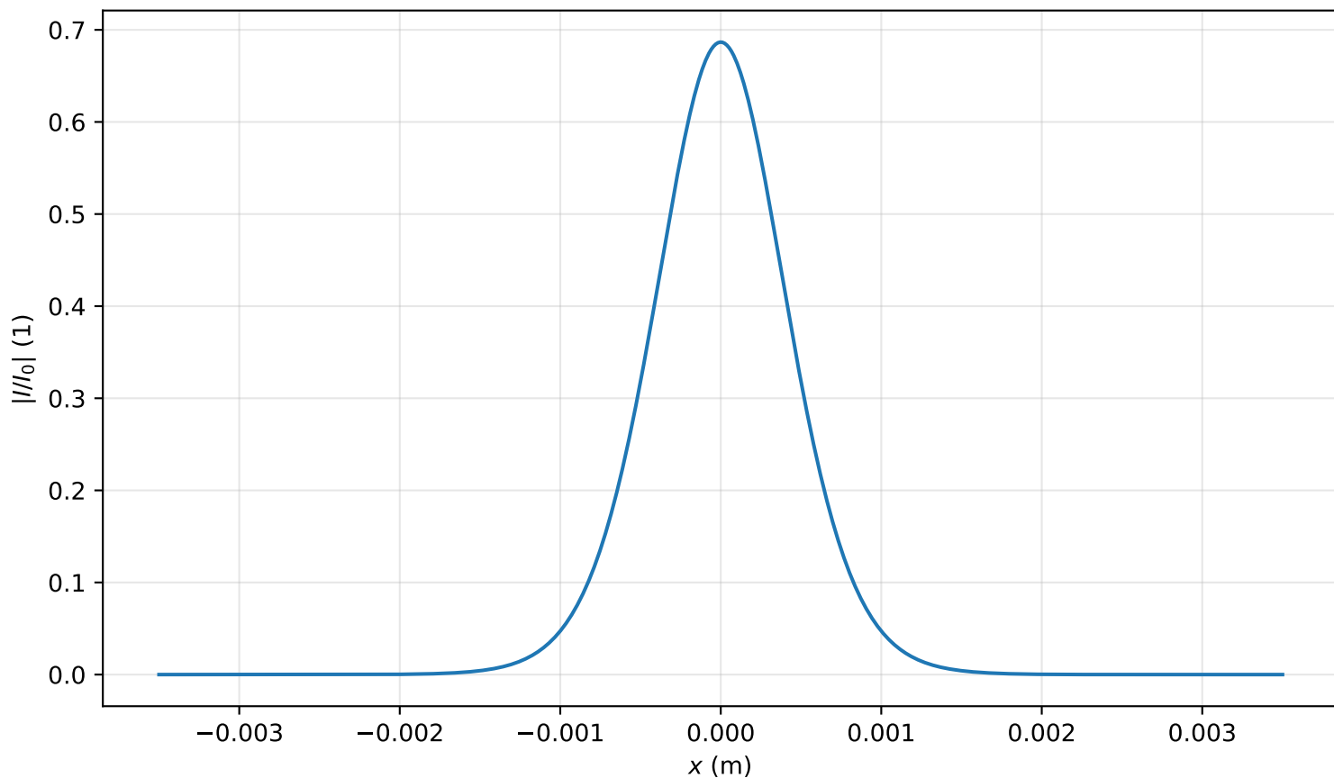
Intensity profile I(x, y = 0, z = 2.149m)/I_0 , P_{in}=0.4P_{cr} , artificial time
